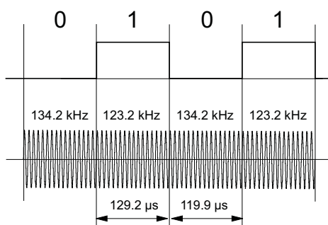
Figure 1-2. FM Principle Used for the Read Function of TI-RFid™ Transponders
